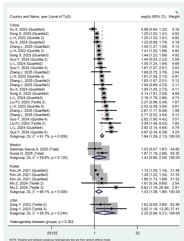
Figure 3. Forest plot showing the association between TyG index and risk of GDM by country.
